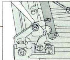
7. Apply the oil to the shift key pivot screws (found on many portables).
